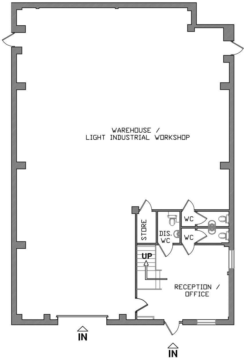
GROUND FLOOR
