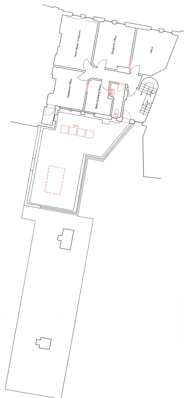
Second Floor 1:100
