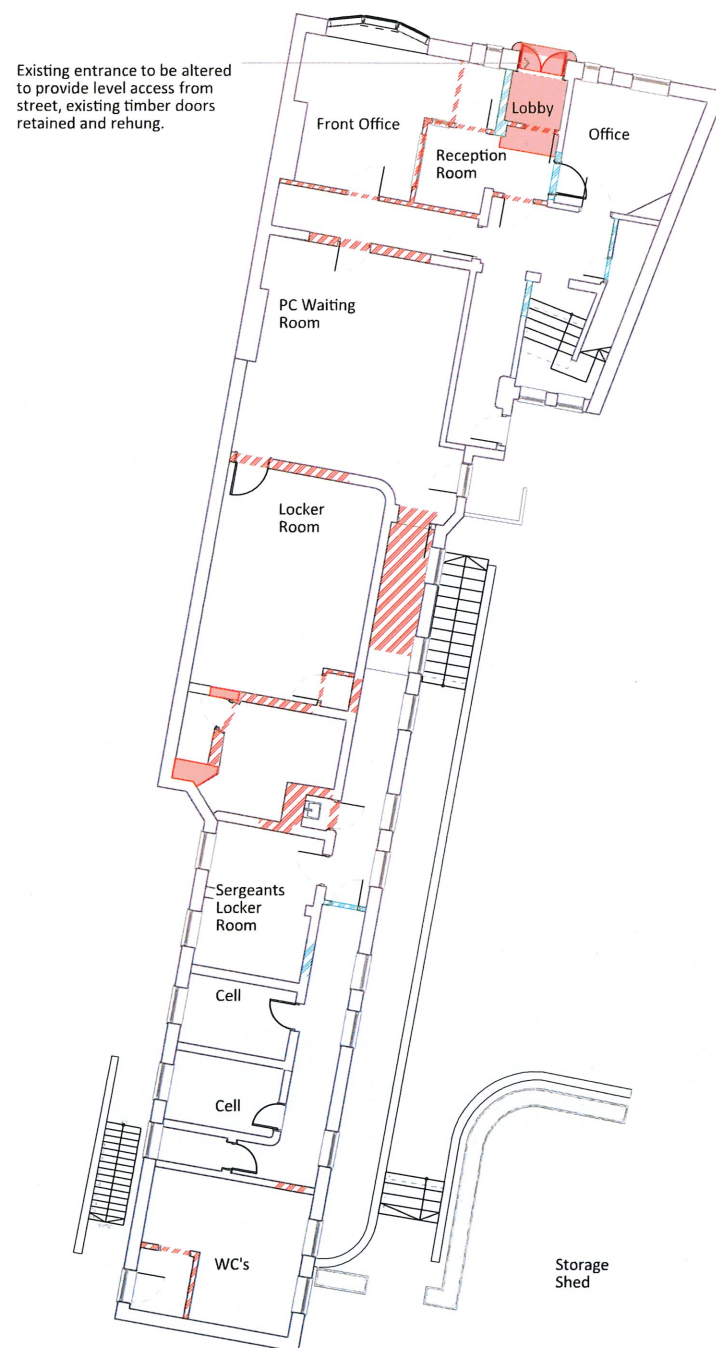
Ground Floor 1:100
