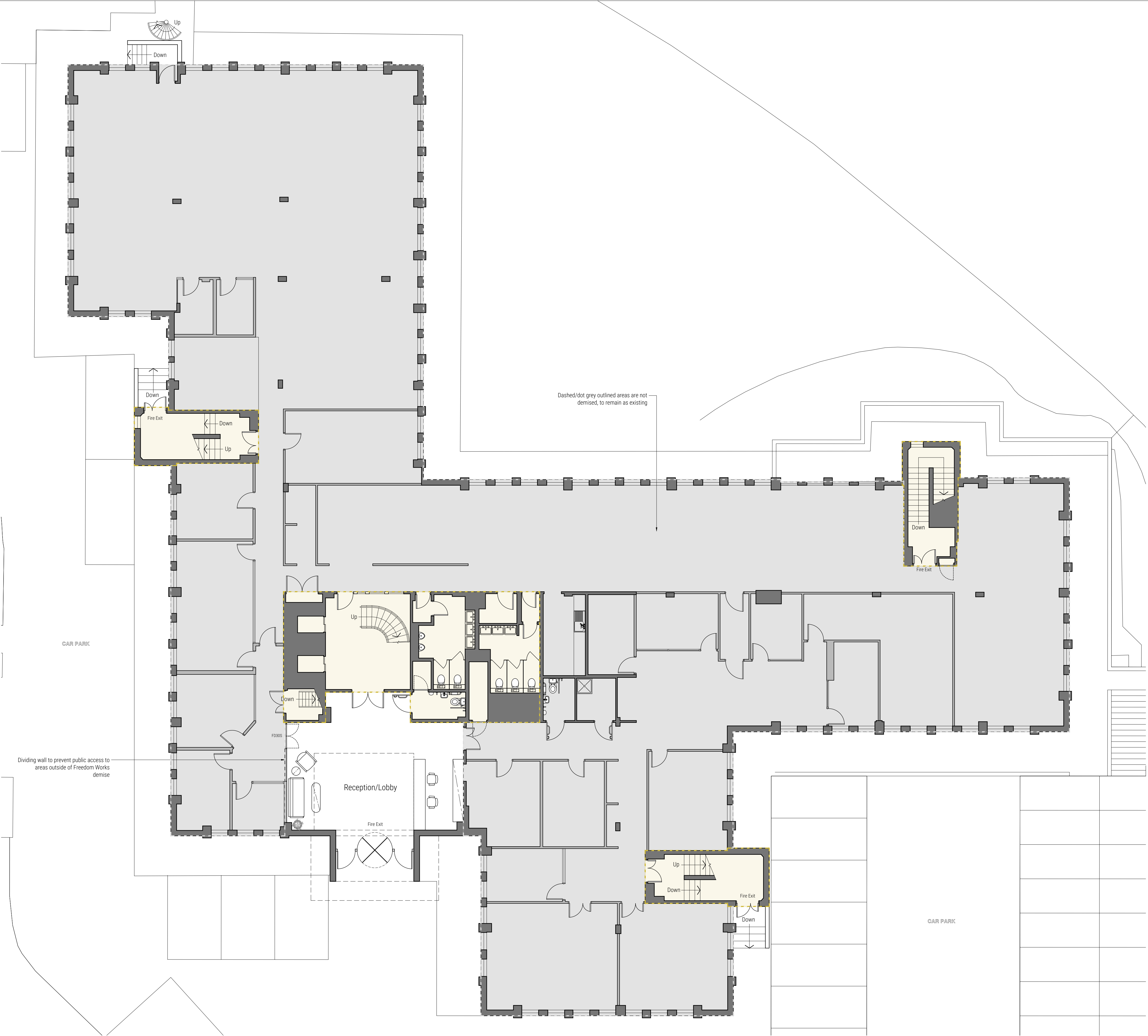
Proposed Ground Floor General Arrangement Plan
